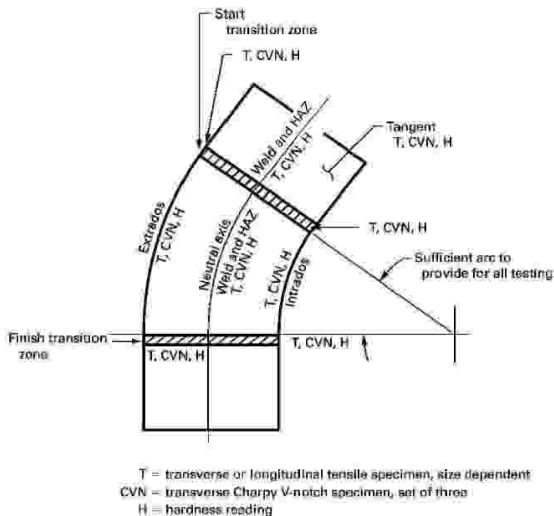
Figure 2 Test Specimen Locations and Orientations — Longitudinal Seam
