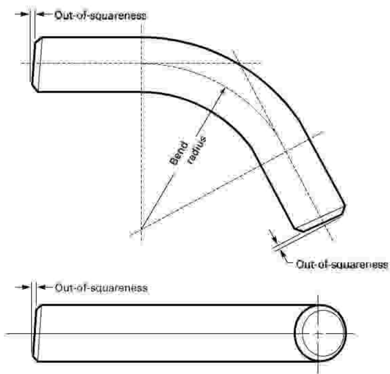
(b) Measurement of Out-of-Squareness
