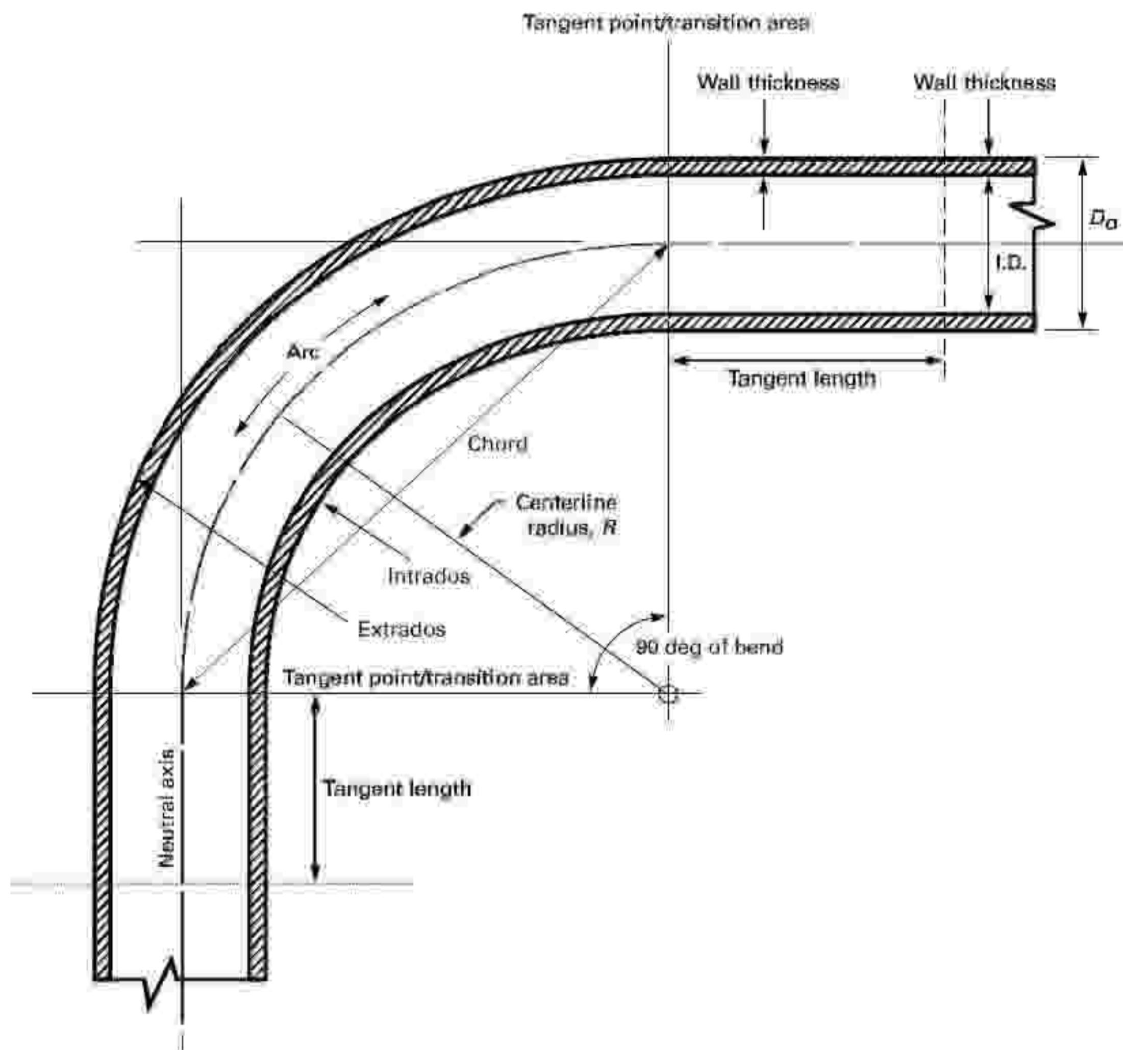
Figure 1 Bend Dimensional Terms
