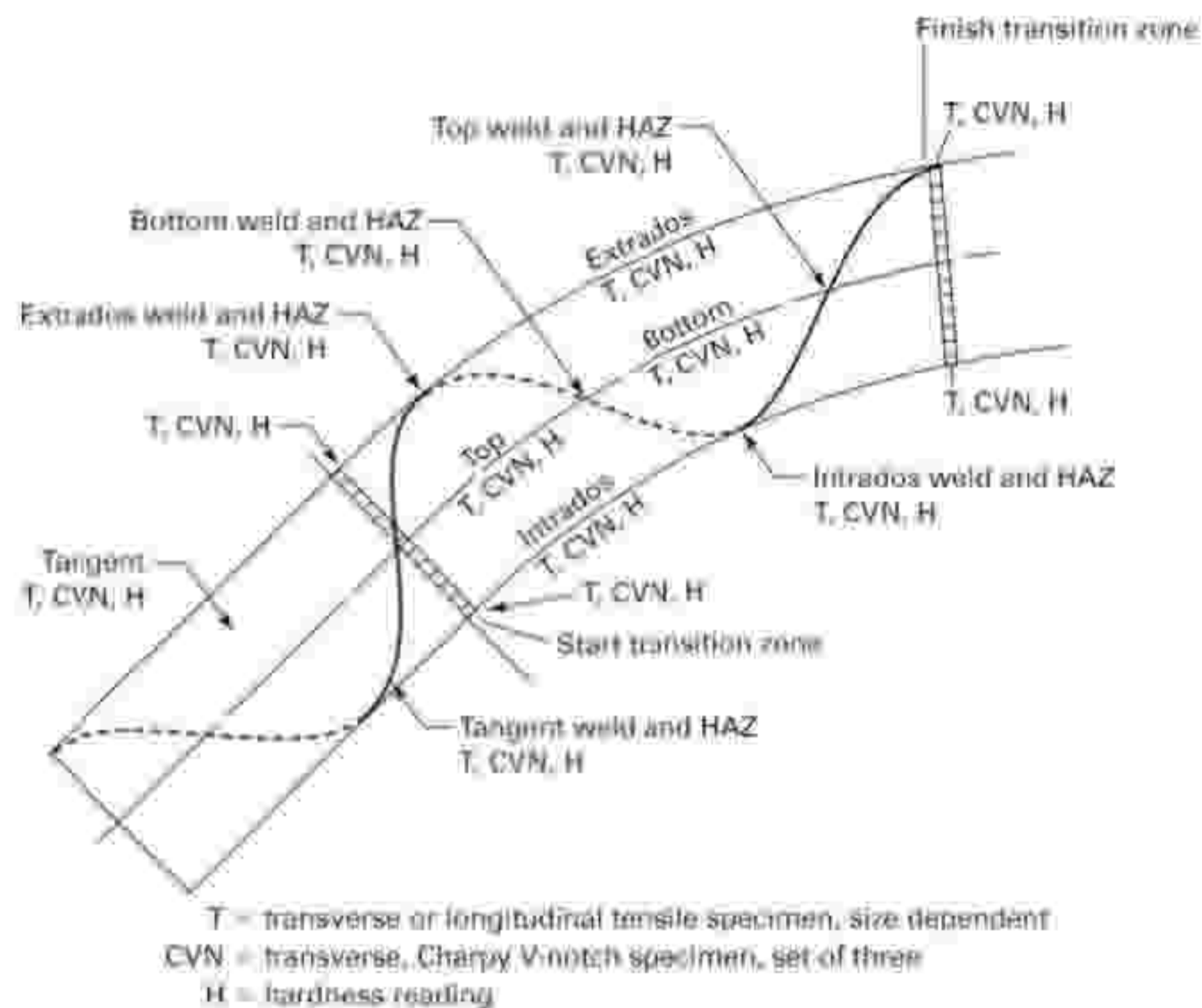
Figure 3 Test Specimen Locations and Orientations — Helical Seam
