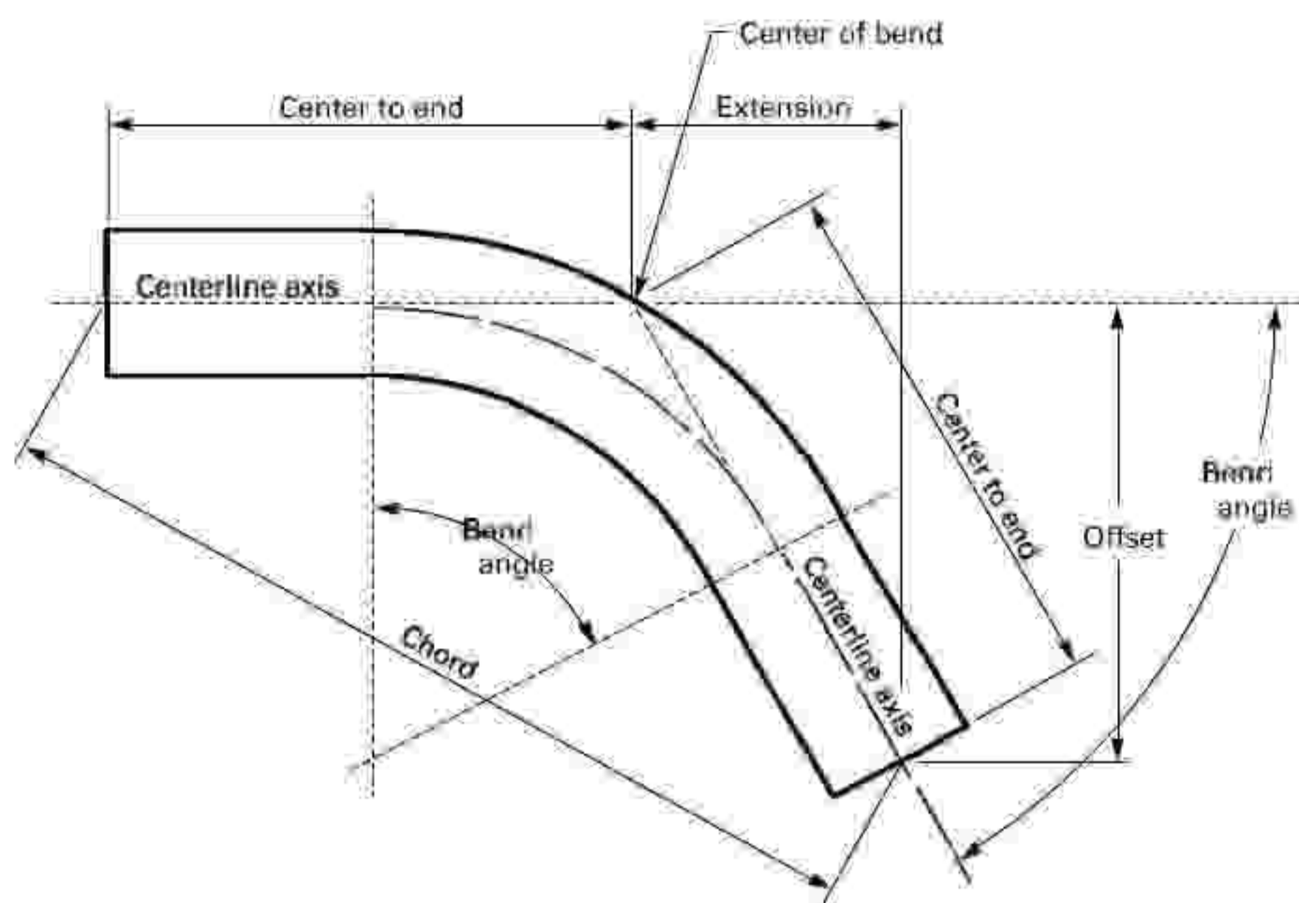
Figure 4 Measurement of Bend Angle and Out-of-Squareness
