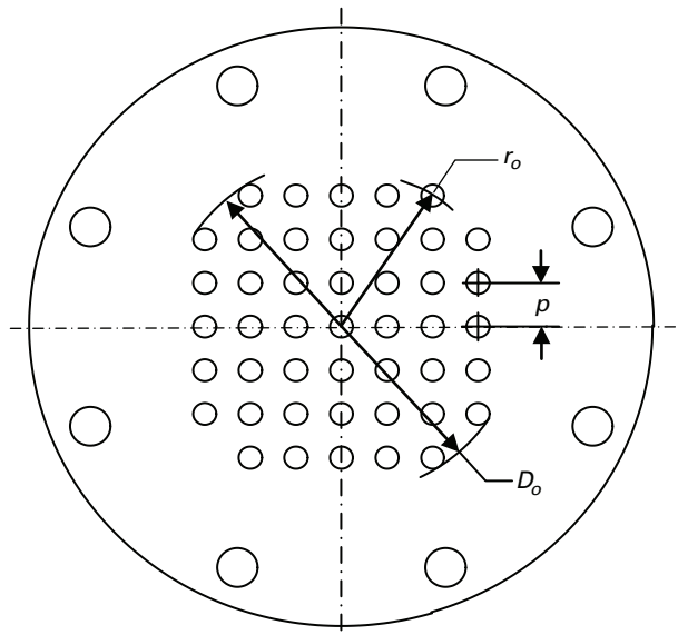
(c) Square Element Pattern
