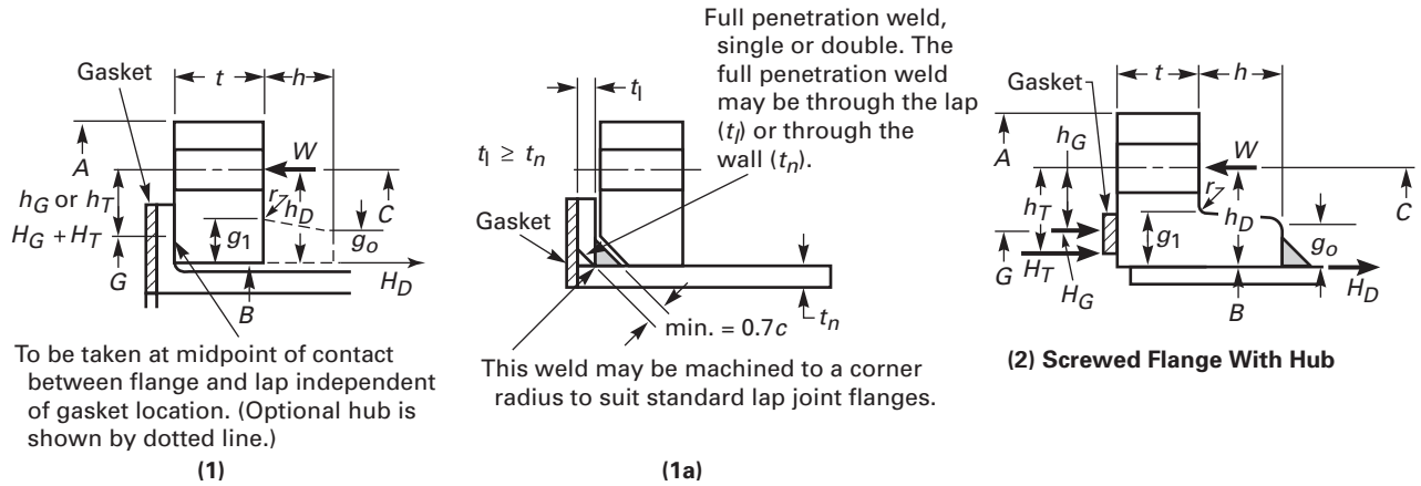
Figure 2-4 Types of Flanges
