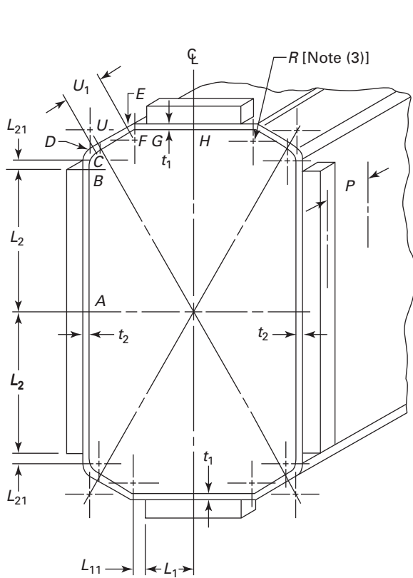
Figure 13-2(a) Vessels of Rectangular Cross Section (Cont'd)
