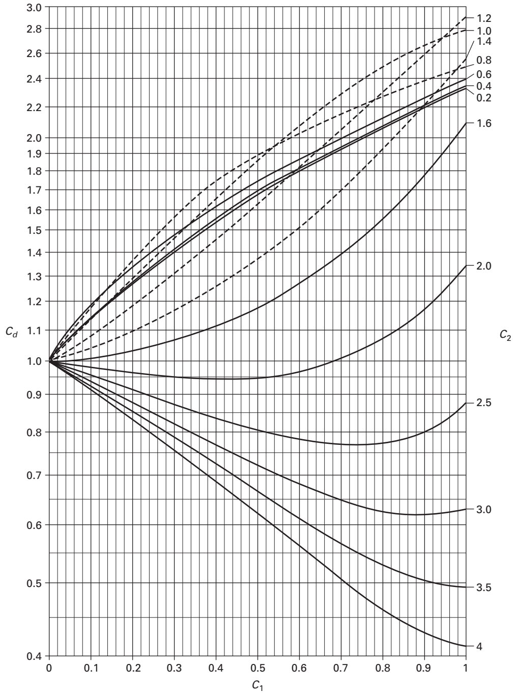
Figure 26-6 Coefficient C_d
