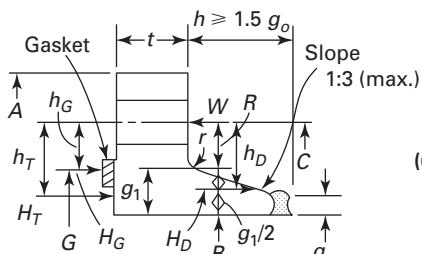
Figure 2-4 Types of Flanges (Cont'd)
