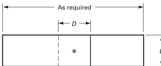
Figure 17-7 Single-Spot-Weld Tension Specimen, Two-Ply Joint
