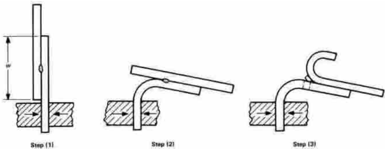
Figure 17-16 Peel Test
