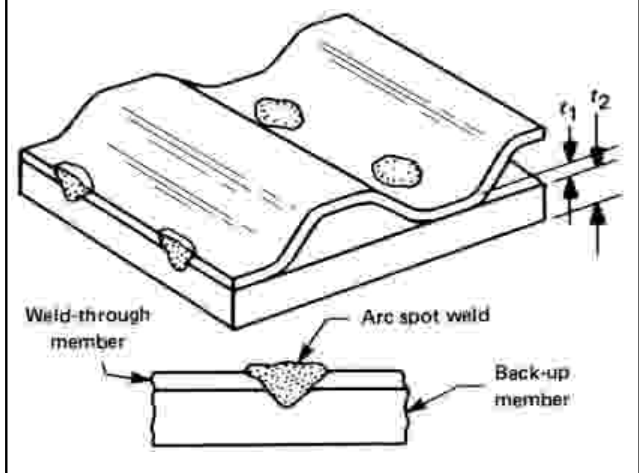
Figure 17-4 Arc-Spot-Welded Two-Layer Assembly
