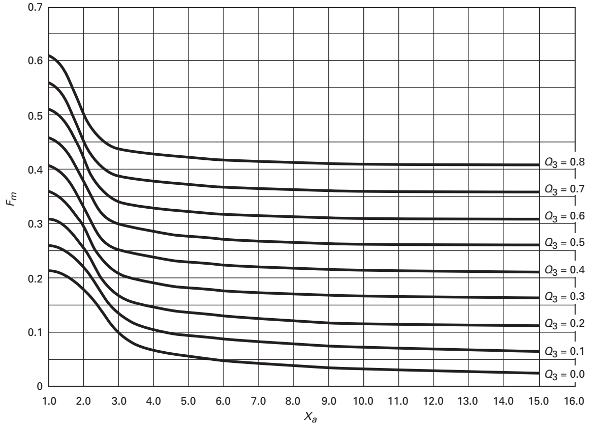
Figure UHX-13.5.7-1 F_m Versus X_a ( 0.0 \leq Q_3 \leq 0.8 )
