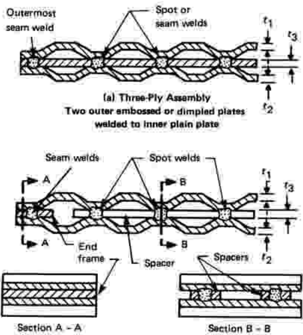
Figure 17-6 Three-Ply Assemblies
