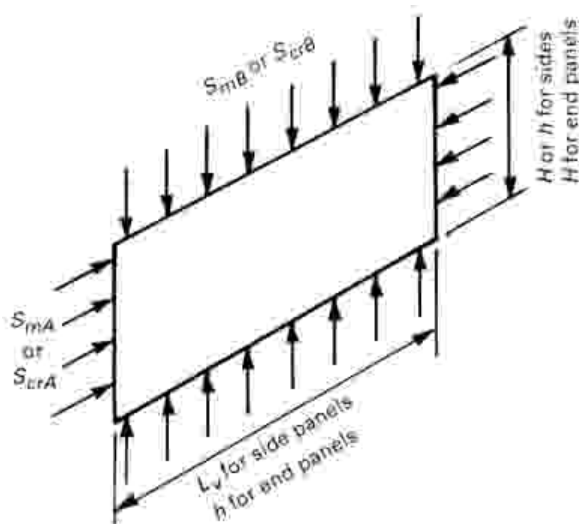
Figure 13-14(b) Orientation of Panel Dimensions and Stresses
